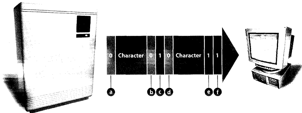
Fig 3 Asynchronous transmission
