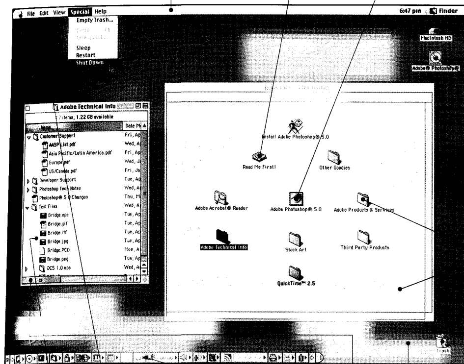
Fig 2 Mac GUI
