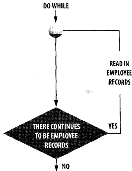
Fig 2 While loop
