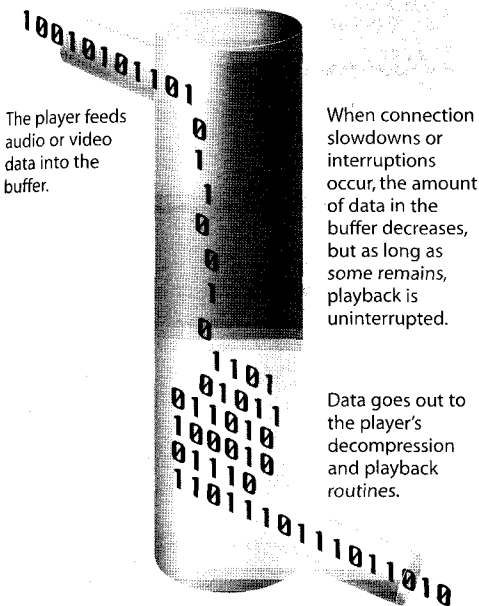
Fig 3 Video buffering
